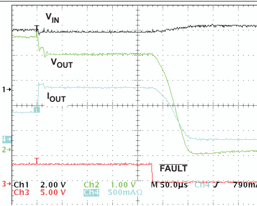
Figure 19. OCP, Powering Up into a Short Circuit on OUT Pin, OCP Counter Counts to 15 Before Switching OFF the Device
