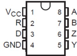
Figure 3-1. D, PS, or P Package Top View
