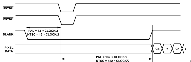
Figure 29. Timing Mode 2 Even-to-Odd Field Transition Main/Subordinate
