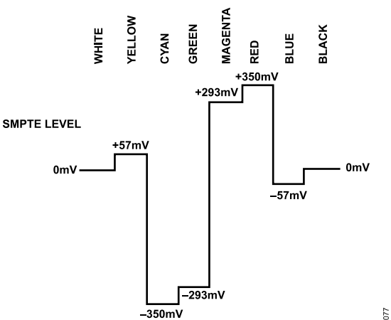
Figure 78. PAL 100% Color Bars, Pr Levels
