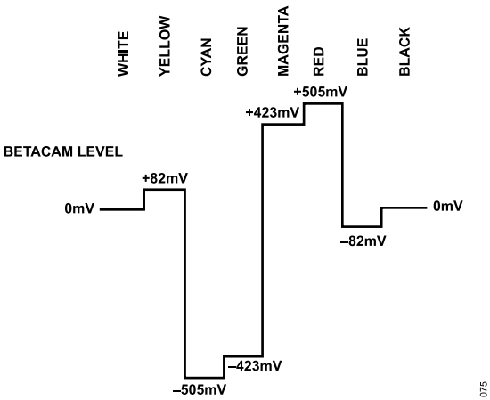
Figure 76. NTSC 100% Color Bars, No Pedestal Pr Levels
