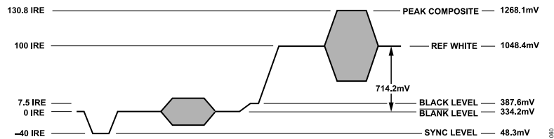
Figure 61. NTSC Composite Video Levels
