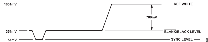
Figure 70. PAL Luma Video Levels
