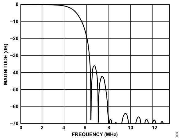
Figure 7. PAL Low-Pass Luma Filter
