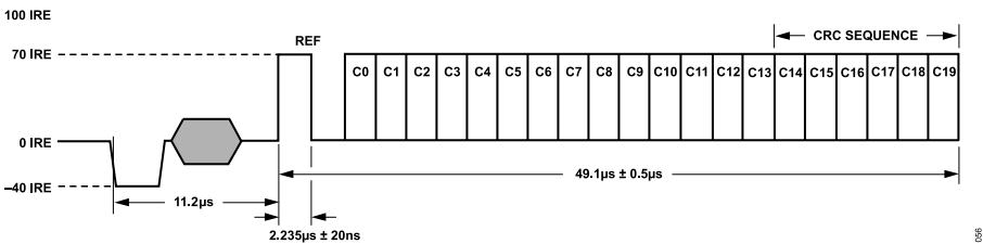
Figure 57. CGMS Waveform Diagram
