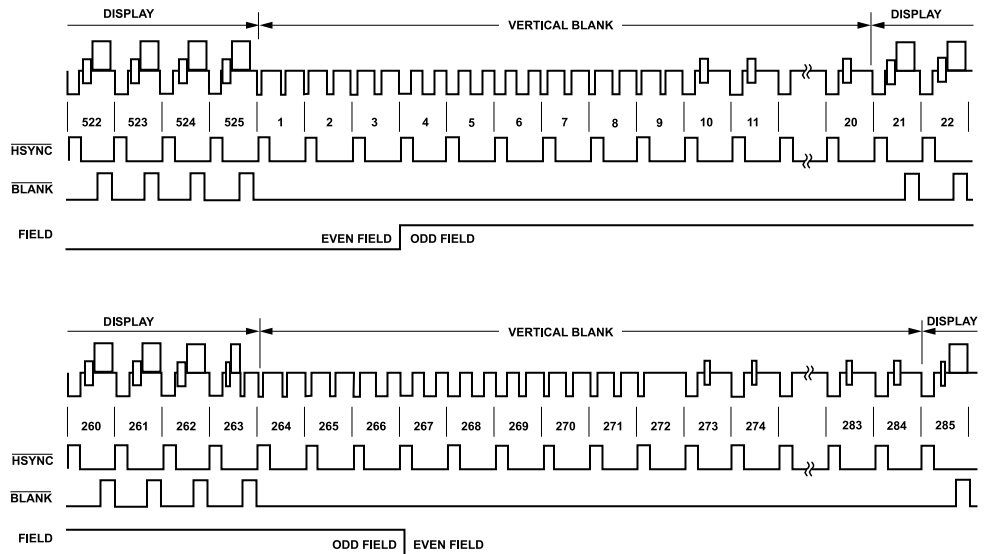
Figure 31. Timing Mode 3 (NTSC)
