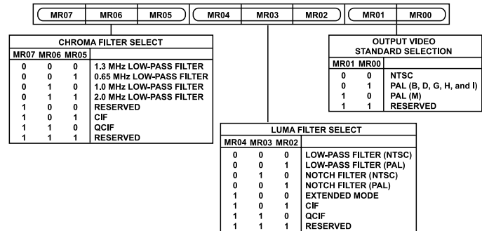
Figure 38. Mode Register 0
