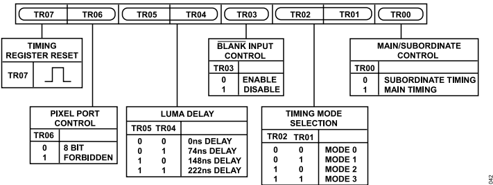
Figure 43. Timing Register 0
