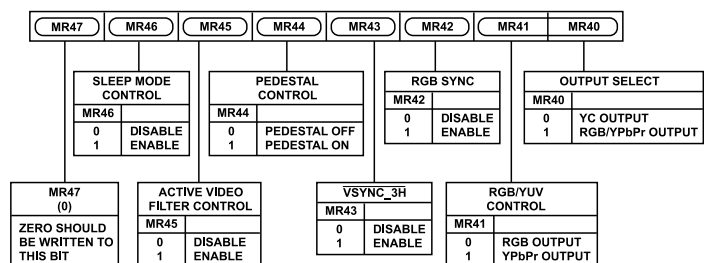
Figure 42. Mode Register 4
