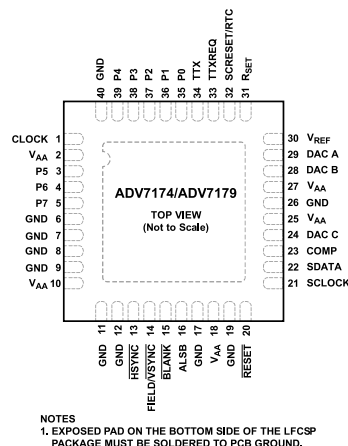
Figure 5. Pin Configurations
