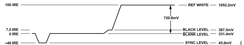
Figure 64. NTSC RGB Video Levels
