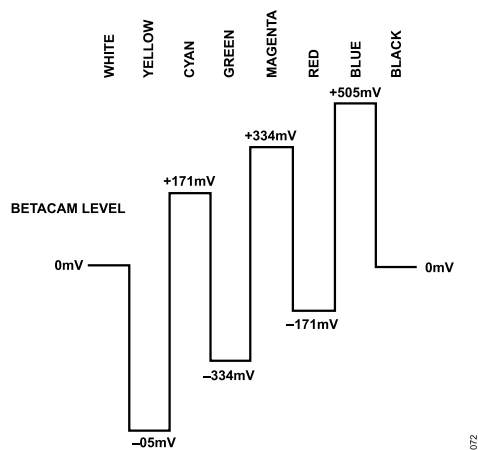
Figure 73. NTSC 100% Color Bars, No Pedestal Pb Levels
