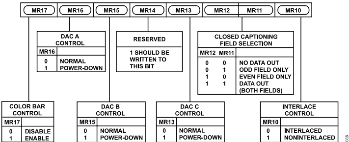
Figure 39. Mode Register 1
