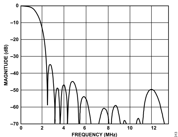
Figure 13. 1.3 MHz Low-Pass Chroma Filter
