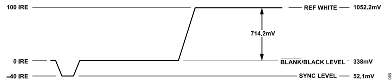
Figure 66. NTSC Luma Video Levels
