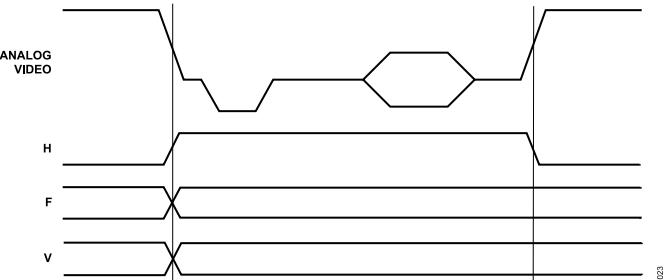
Figure 23. Timing Mode 0 Data Transitions (Main Mode)
