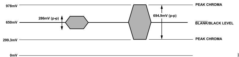
Figure 67. NTSC Chroma Video Levels
