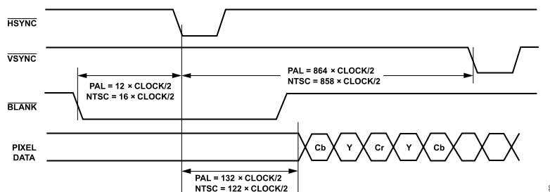
Figure 30. Timing Mode 2 Odd-to-Even Field Transition Main/Subordinate
