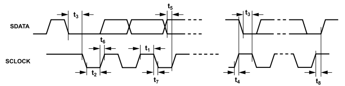
Figure 2. MPU Port Timing Diagram
