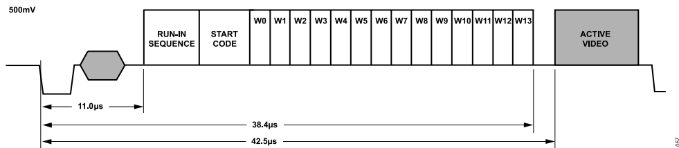
Figure 58. WSS Waveform Diagram
