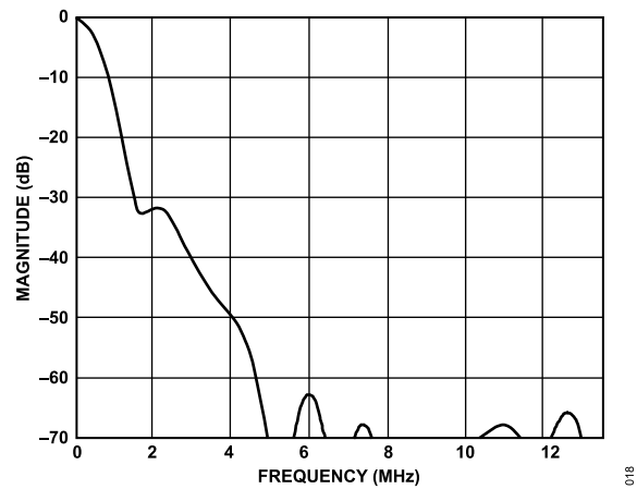
Figure 18. QCIF Chroma Filter
