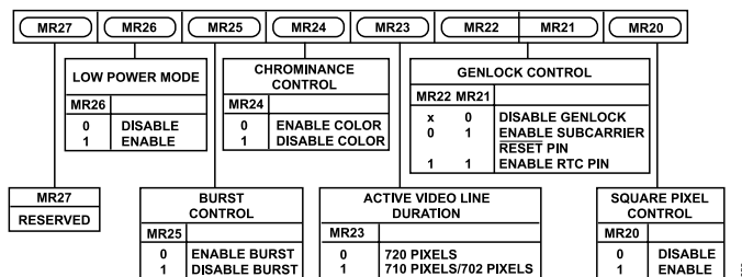
Figure 40. Mode Register 2
