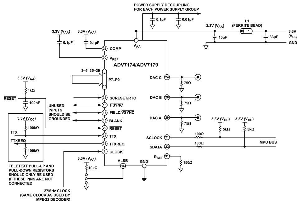
Figure 54. Recommended Analog Circuit Layout
