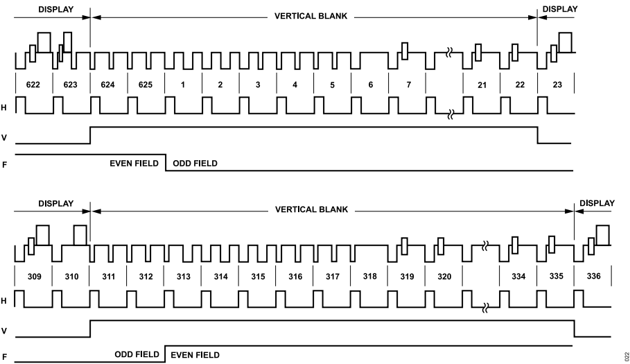
Figure 22. Timing Mode 0 (PAL Main Mode)
