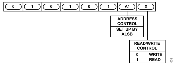
Figure 34. ADV7179 Address
