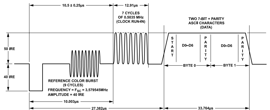
Figure 56. Closed Captioning Waveform (NTSC)
