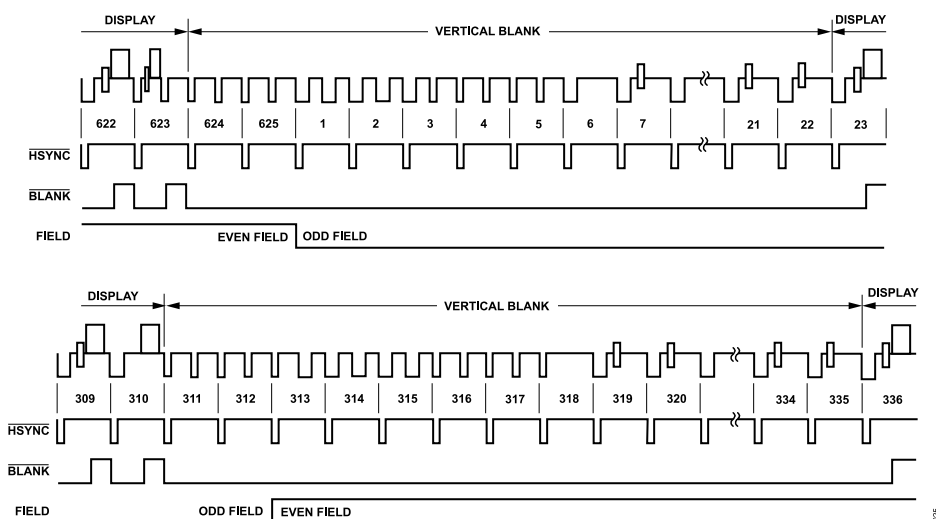
Figure 25. Timing Mode 1 (PAL)
