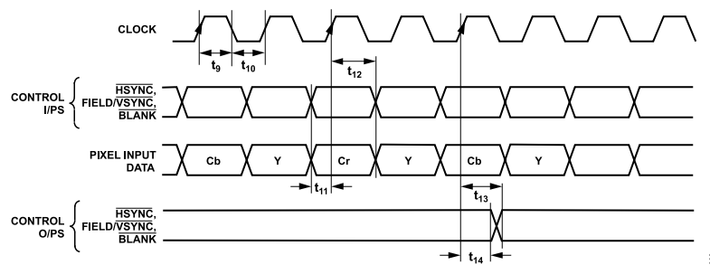
Figure 3. Pixel and Control Data Timing Diagram
