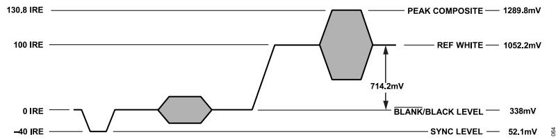
Figure 65. NTSC Composite Video Levels
