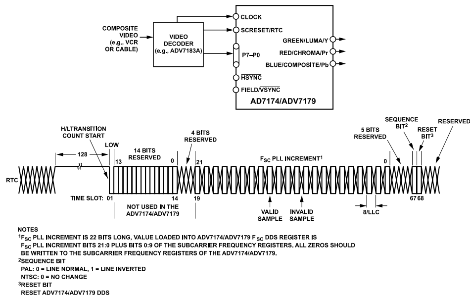
Figure 19. RTC Timing and Connections
