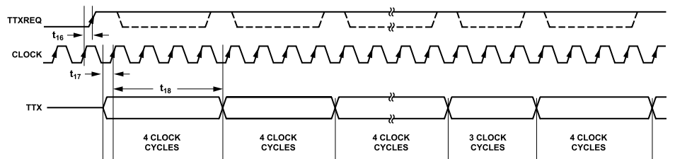
Figure 4. Teletext Timing Diagram
