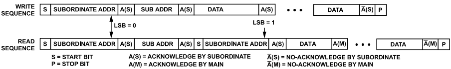
Figure 36. Write and Read Sequences
