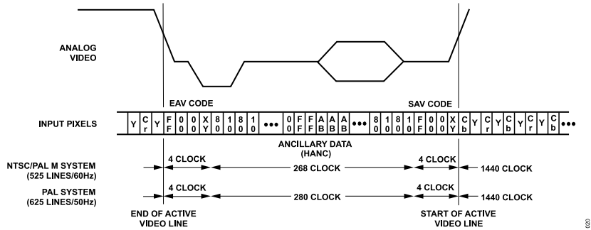
Figure 20. Timing Mode 0 (Subordinate Mode)
