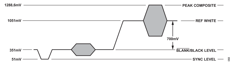
Figure 69. PAL Composite Video Levels
