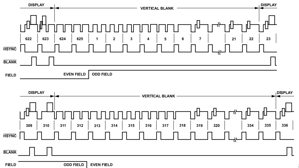
Figure 32. Timing Mode 3 (PAL)
