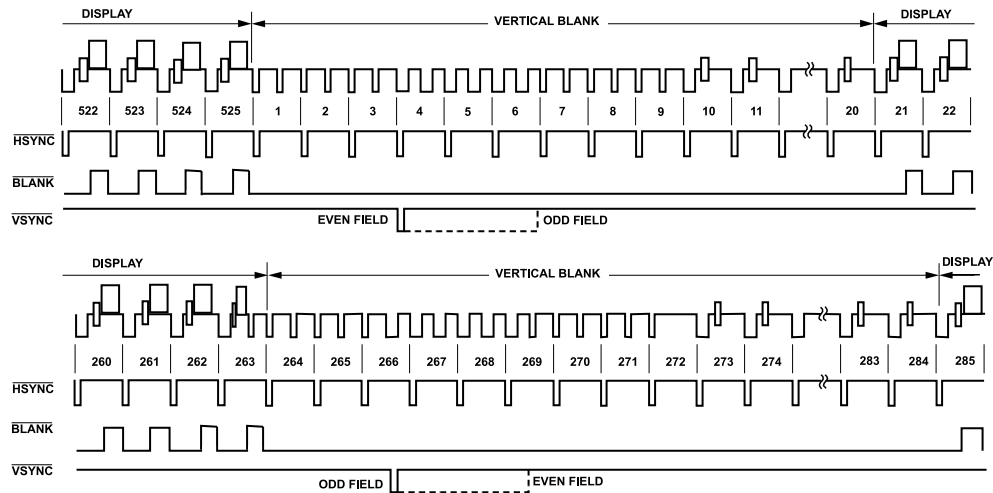
Figure 27. Timing Mode 2 (NTSC)
