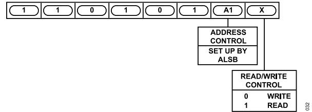
Figure 33. ADV7174 Subordinate Address
