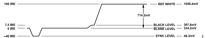
Figure 62. NTSC Luma Video Levels
