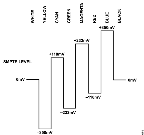
Figure 75. PAL 100% Color Bars, Pb Levels
