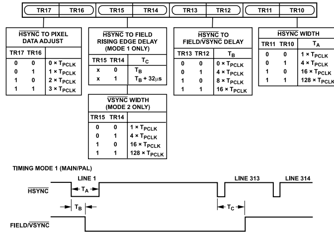
Figure 44. Timing Register 1
