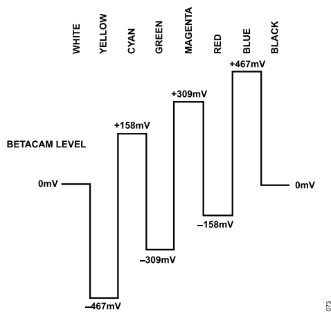
Figure 74. NTSC 100% Color Bars with Pedestal Pb Levels
