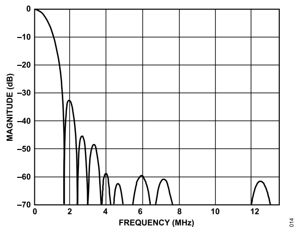
Figure 14. 0.65 MHz Low-Pass Chroma Filter
