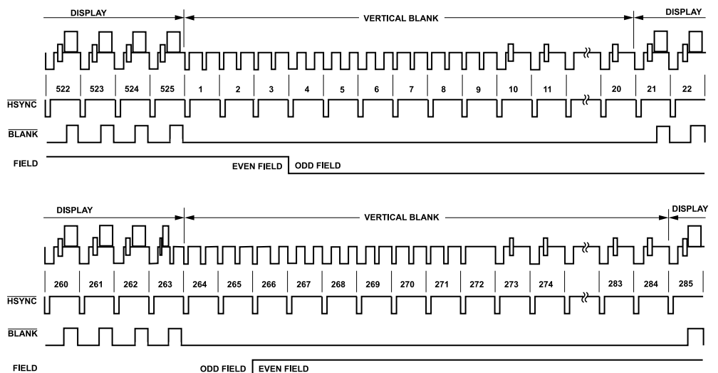
Figure 24. Timing Mode 1 (NTSC)
