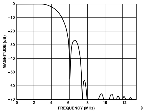
Figure 6. Chrominance Internal Filter Specifications
