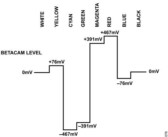
Figure 77. NTSC 100% Color Bars with Pedestal Pr Levels
