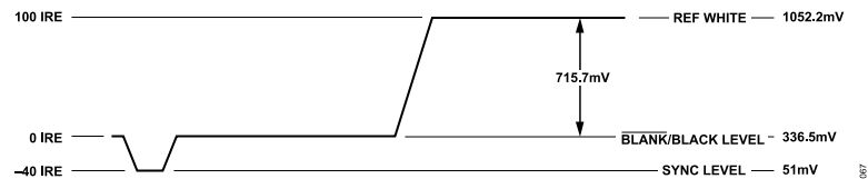
Figure 68. NTSC RGB Video Levels
