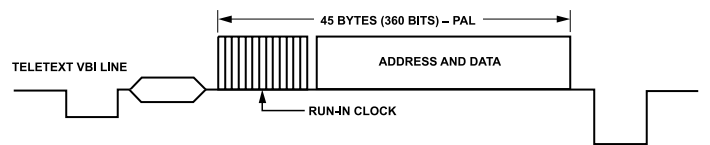
Figure 59. Teletext VBI Line
