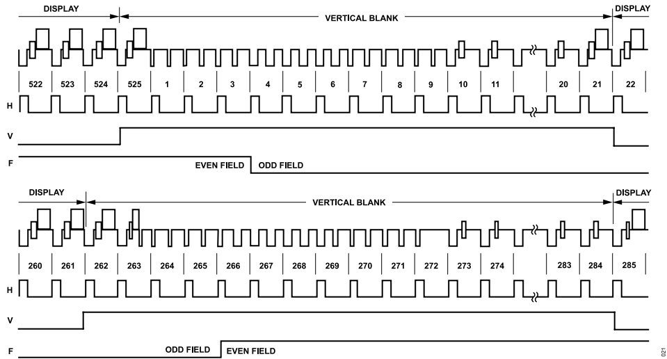
Figure 21. Timing Mode 0 (NTSC Main Mode)
