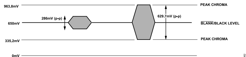
Figure 63. NTSC Chroma Video Levels
