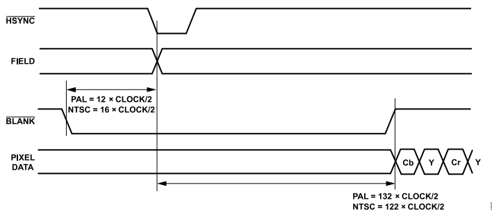
Figure 26. Timing Mode 1 Odd/Even Field Transitions Main/Subordinate
