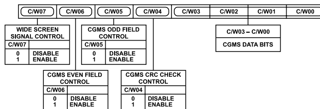
Figure 51. CGMS_WSS Register 0
