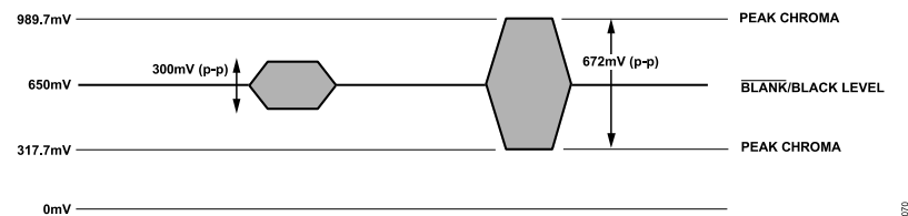
Figure 71. PAL Chroma Video Levels
