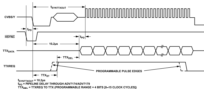
Figure 60. Teletext Functionality
