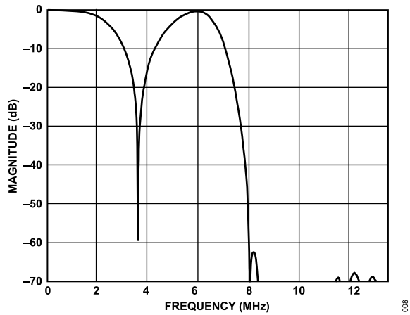
Figure 8. NTSC Notch Luma Filter
