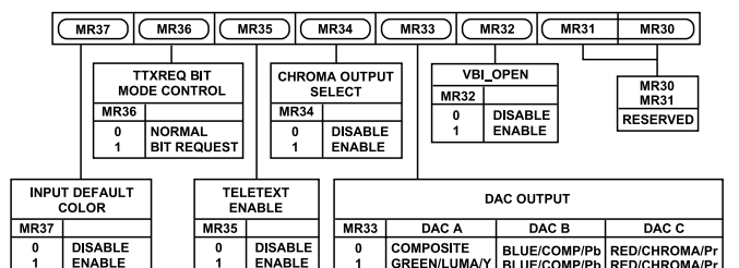
Figure 41. Mode Register 3
