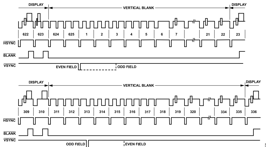
Figure 28. Timing Mode 2 (PAL)
