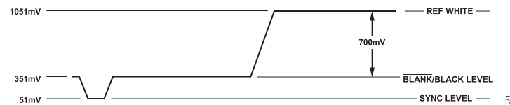
Figure 72. PAL RGB Video Levels
