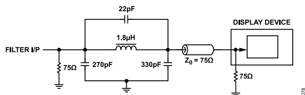
Figure 79. Output Filter
