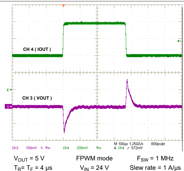
Figure 8-7. Load Transient, 4 A to 8 A, 1 A/μs
