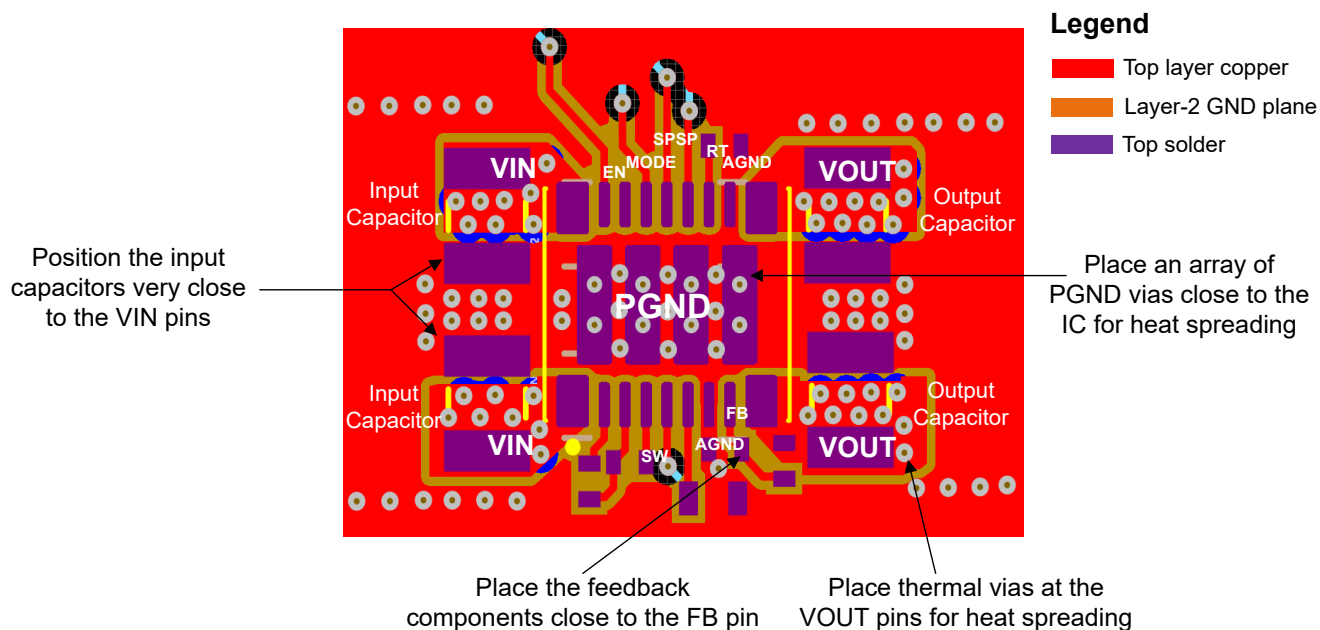
Figure 8-18. Typical Top Layer Design
