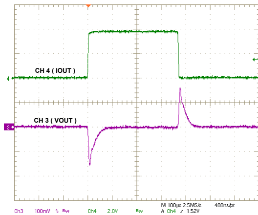
Figure 8-8. Load Transient, 0 A to 4 A, 1 A/μs
