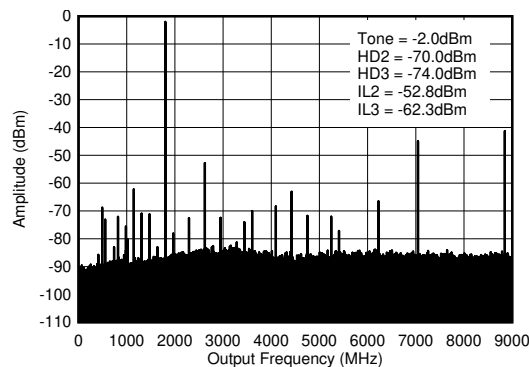
f_{\text{DAC}} = 8847.36\text{MSPS} , interleave mode, 1.8 GHz matching, includes PCB and cable losses. IL_n = f_s/n \pm f_{\text{OUT}} . Figure 5-343. TX Single Tone (-6 dBFS) Output Spectrum at 1.8 GHz ( 0-f_{\text{DAC}} )
