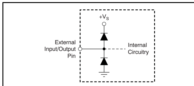
Figure 56. Internal ESD Protection
