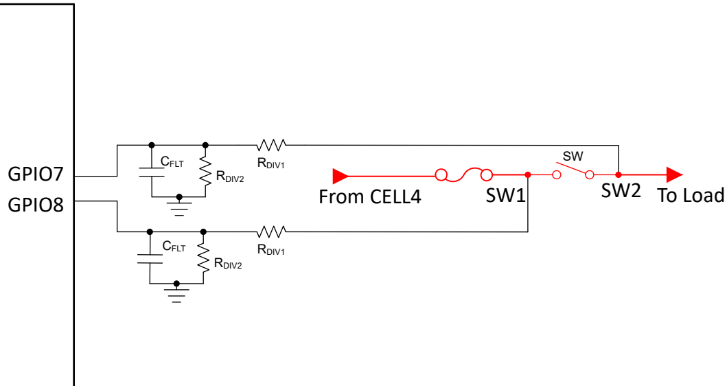
Figure 9-5. Fuse and Relay Status Detection
