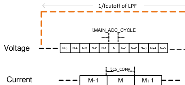
Figure 9-7. Effect of Voltage Low Pass Filter in Continuous Run Mode
