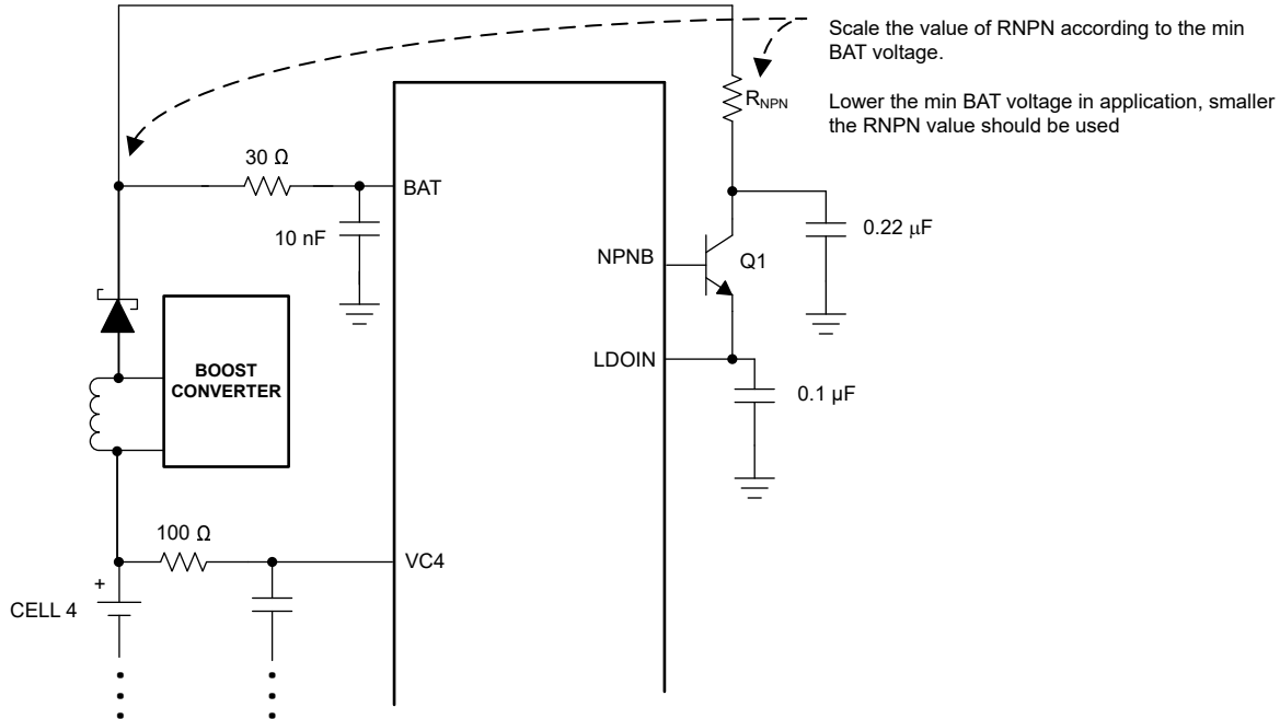
Figure 9-10. Boost Converter to Supply BAT in 4S Applications
