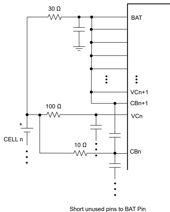
Figure 9-3. Unused VC and CB Channels - 6S
