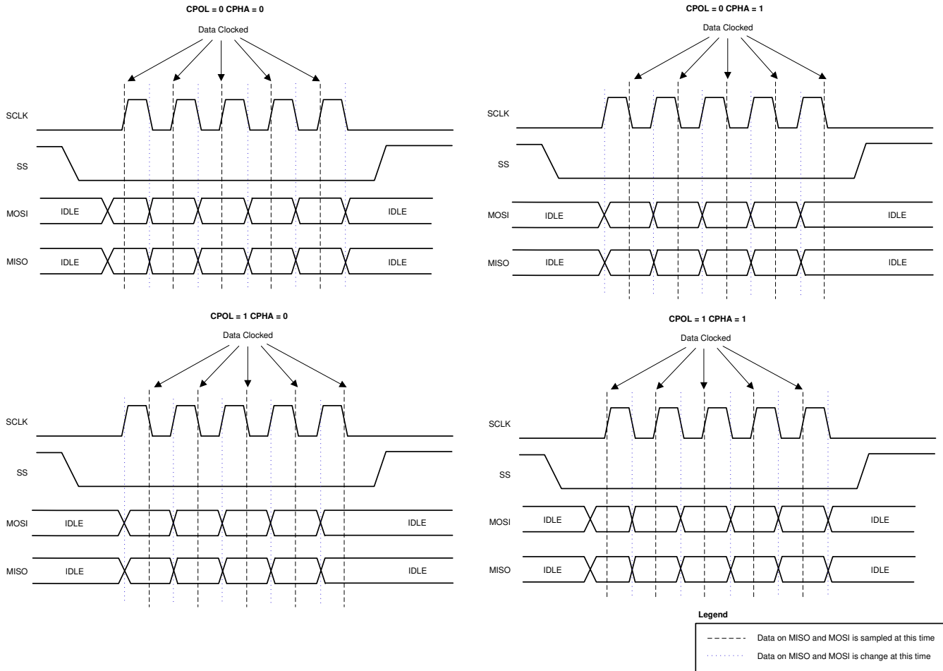
Figure 8-28. SPI Controller CPOL and CPHA
