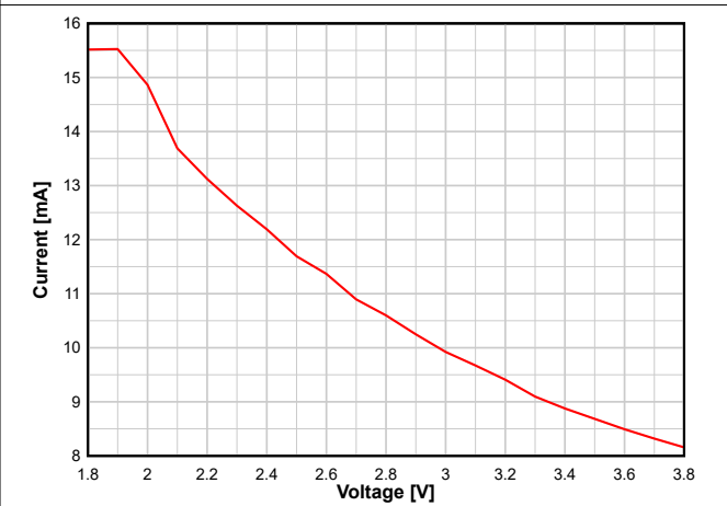
Figure 8-11. TX Current vs. Supply Voltage (VDDS) (BLE 1 Mbps, 2.44 GHz, +5 dBm)
