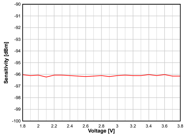
Figure 8-17. Sensitivity vs. Supply Voltage (VDD5) (BLE 1 Mbps, 2.44 GHz, DCDC Off)
