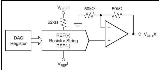
Figure 92. DAC8165 Architecture
