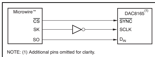
Figure 102. DAC8165 to Microwire Interface
