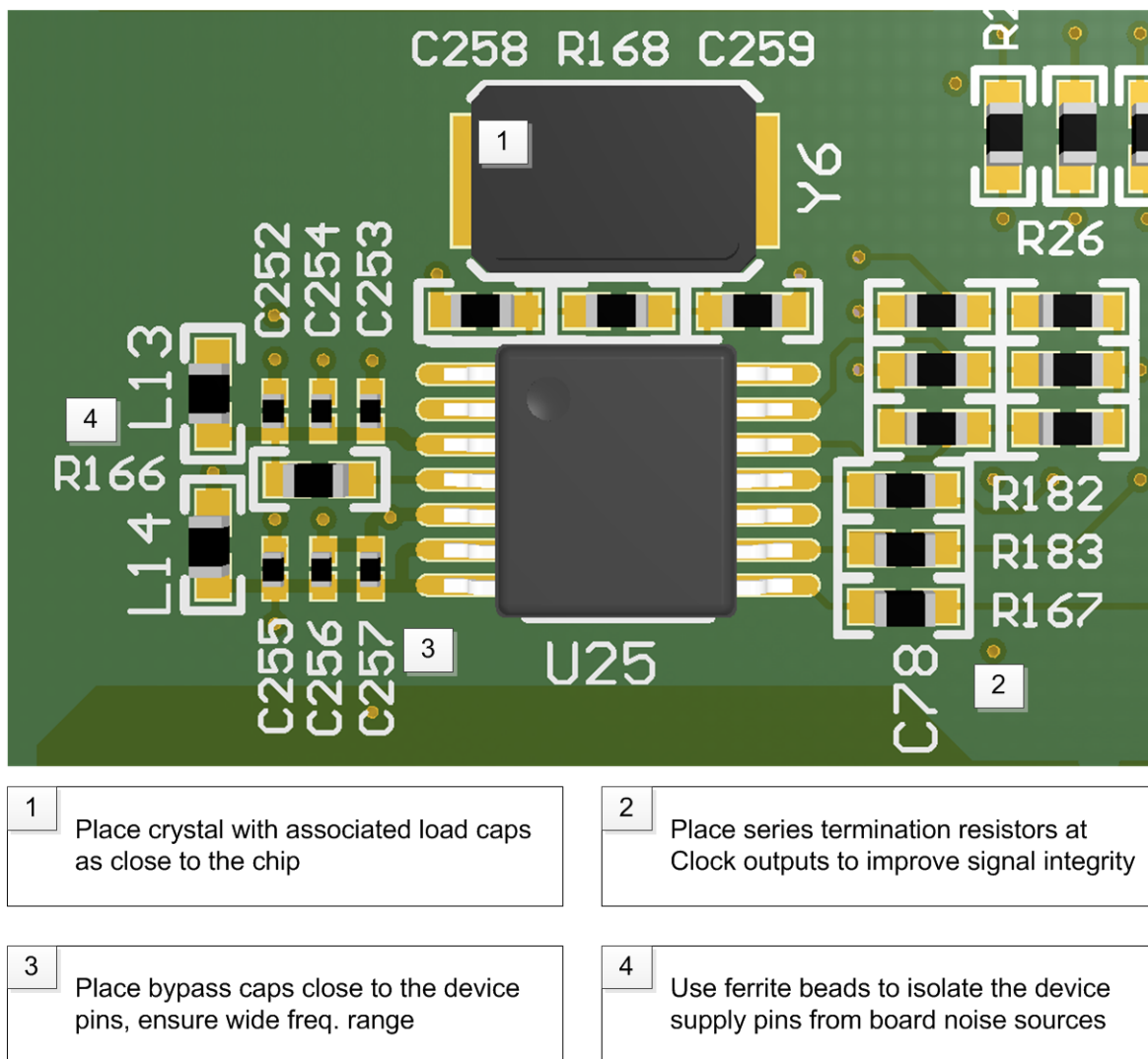
Figure 16. Board Layout
