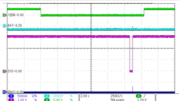
Figure 9-5. Charge Enable
