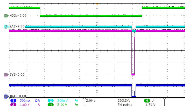
Figure 9-6. Charge Disable
