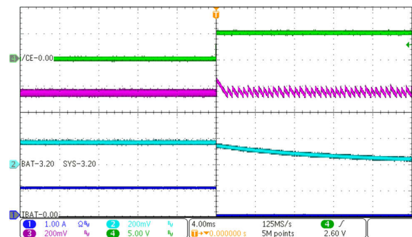
Figure 9-4. Power-Down
