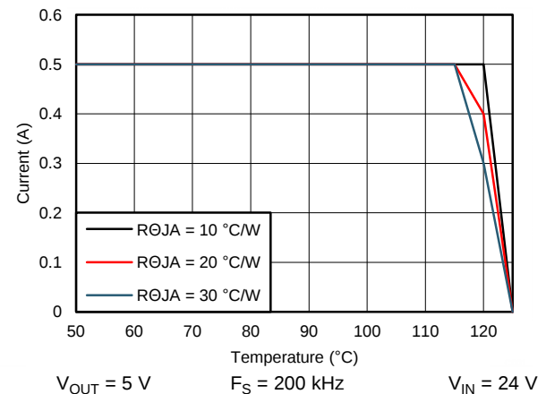
Figure 64. Derating Curve
