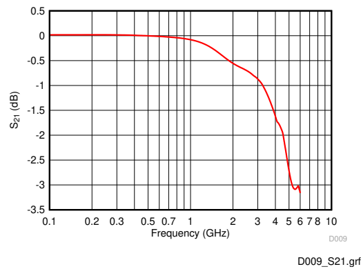
Figure 5-9. Insertion Loss vs. Frequency
