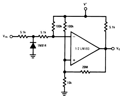
Bi-Stable Multivibrator
