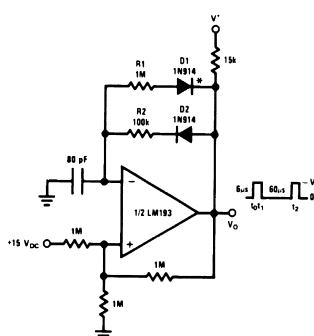
Pulse Generator
