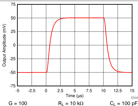
Figure 45. Small-Signal Response
