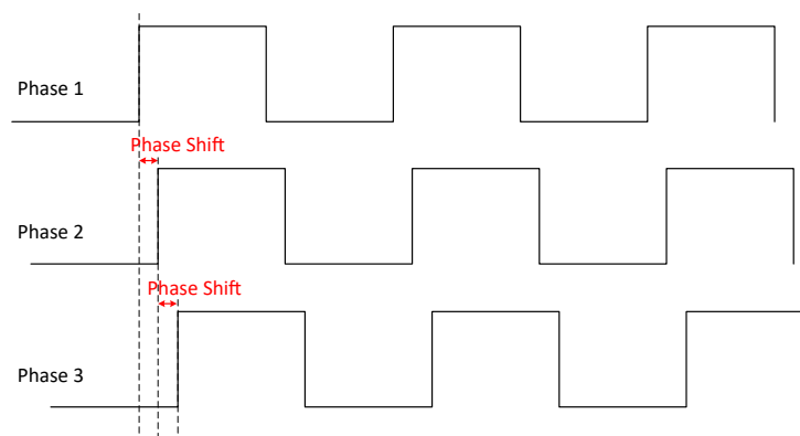
Figure 8-4. Phase Shift
