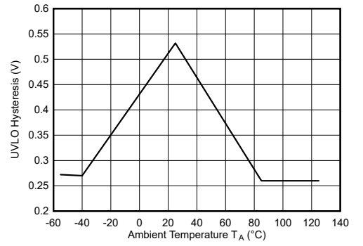
Figure 7-4. V_{CC} UVLO Hysteresis
