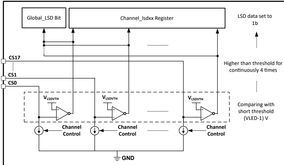
Figure 8-12. LSD Circuit
