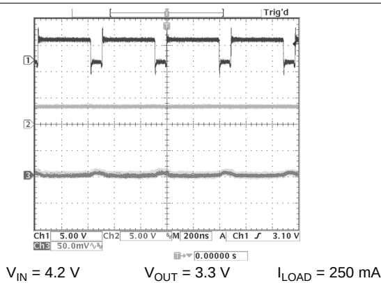
Figure 41. Switch Pins in Buck Mode Operation
