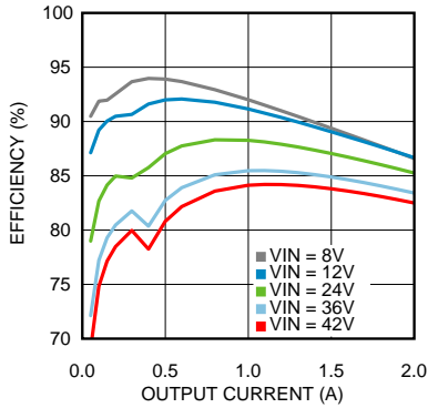
Figure 13. Efficiency V_{OUT} = 5\text{ V} T_A = 85^\circ\text{C}
