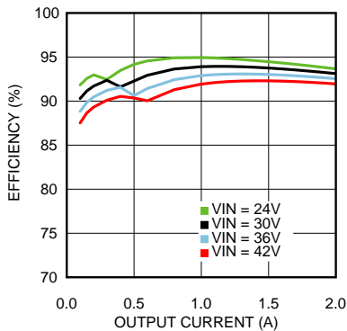
Figure 15. Efficiency V_{OUT} = 12\text{ V} T_A = 85^\circ\text{C}
