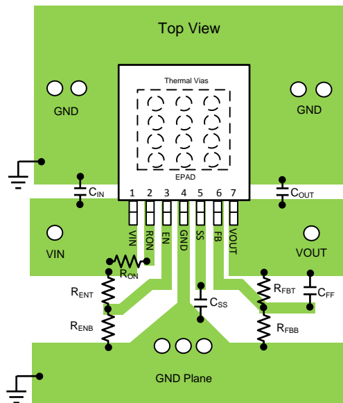
Figure 52. PCB Layout
