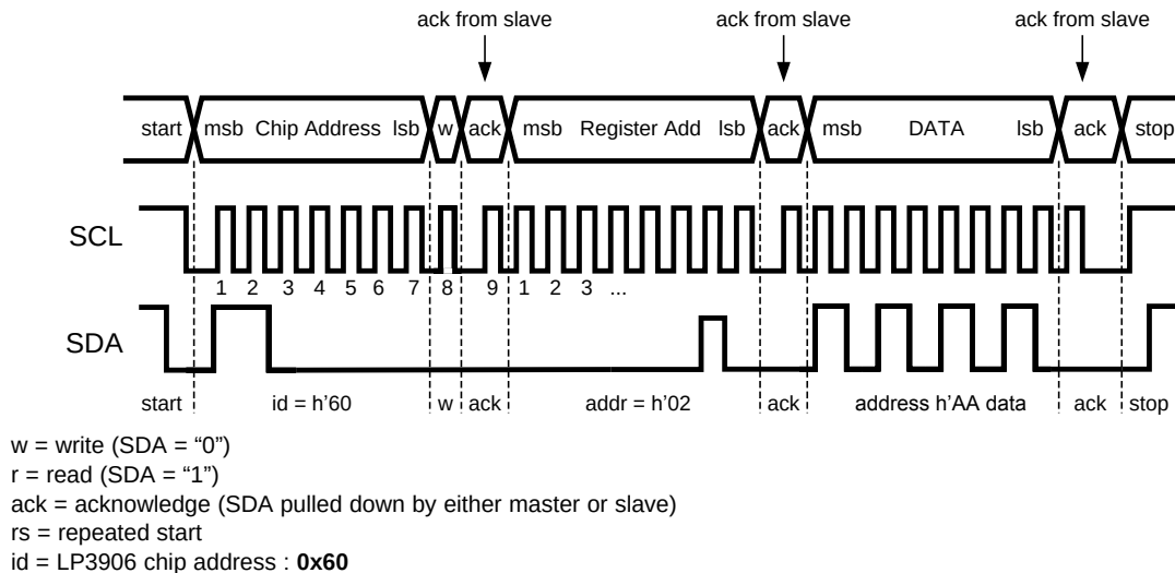
Figure 37. I 2 C Write Cycle
