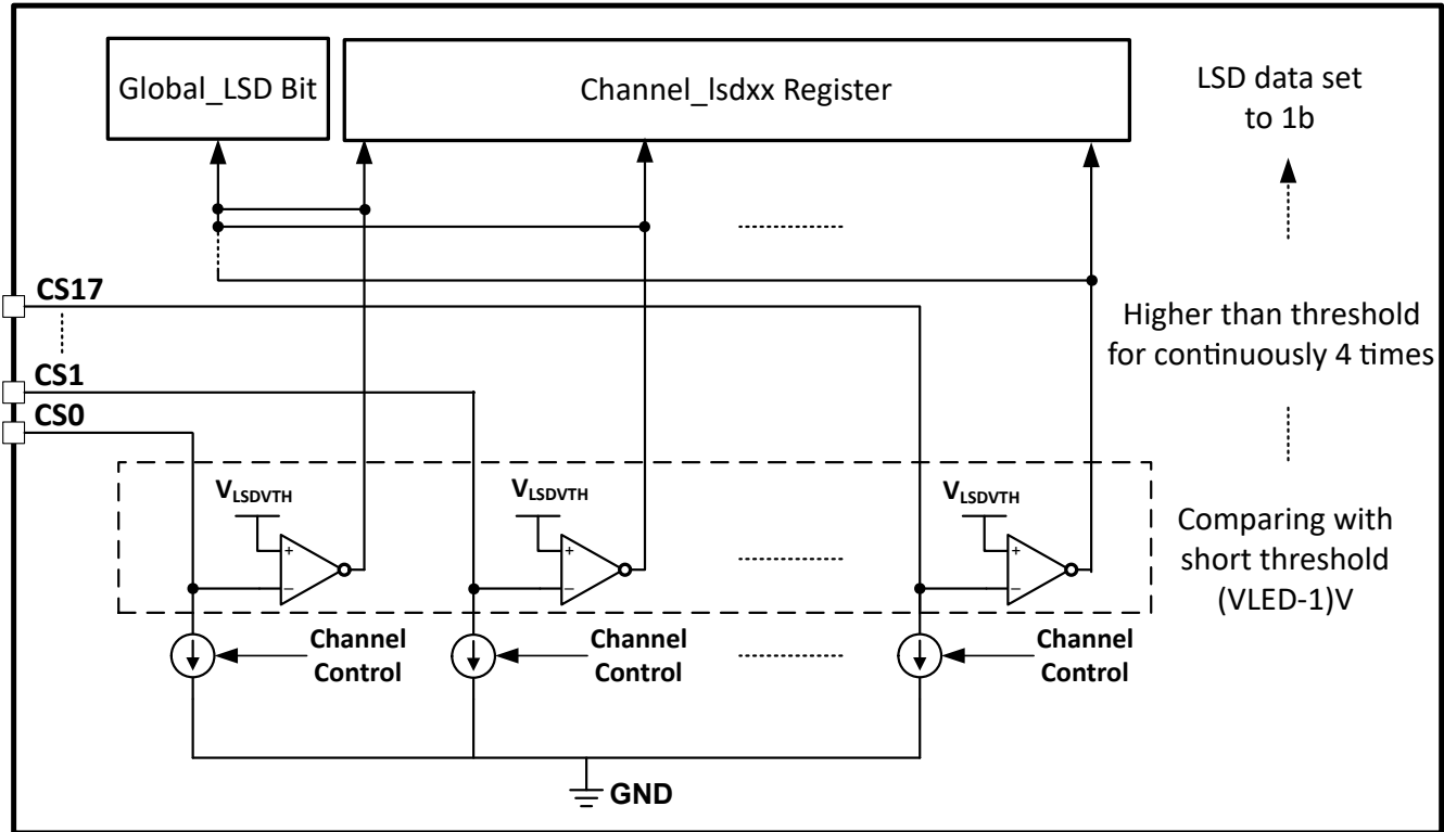
Figure 7-12. LSD Circuit
