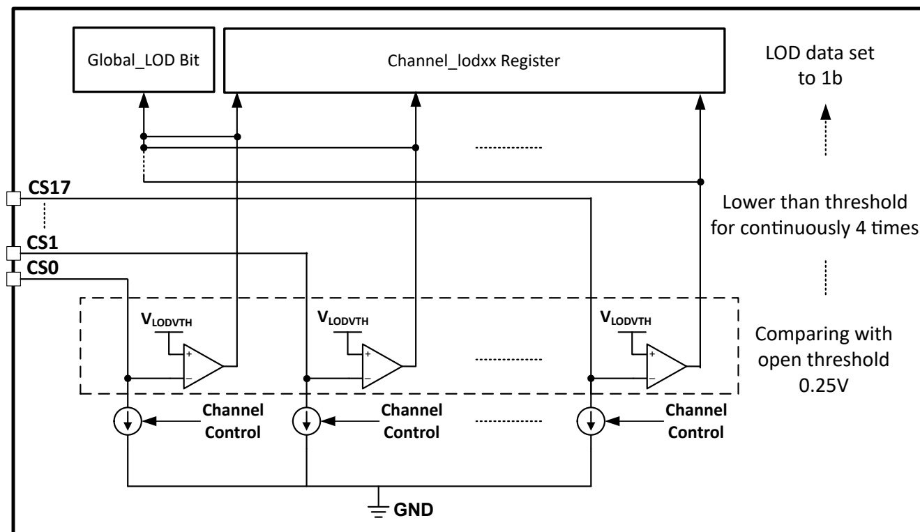
Figure 7-11. LOD Circuits
