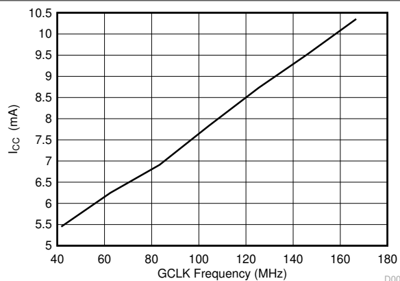
Figure 7-8. Icc Current vs GCLK Frequency
