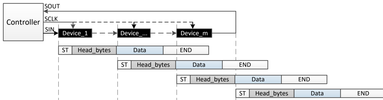
Figure 8-17. Data Write Command With Broadcast
