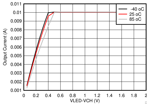
Figure 7-2. Channel Current vs (VLED-Vchannel) Voltage
