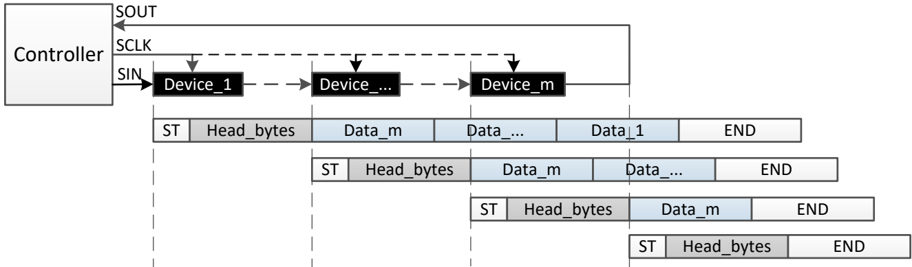
Figure 8-19. Data Write Command With Non-Broadcast
