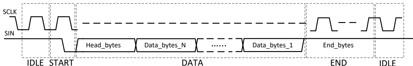
Figure 8-14. CCSI Frame
