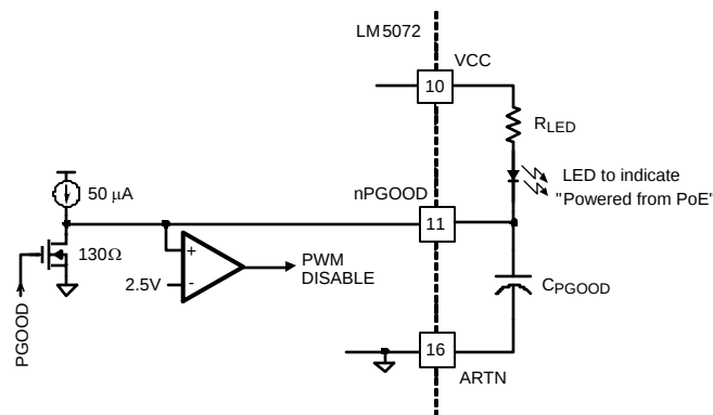
Figure 22. "Powered-from-PoE" Indicator and Power Good Delay Timer
