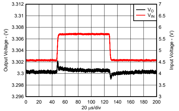
Figure 7-19. Line Transient Response (New Chip)
