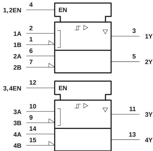
logic symbol†
