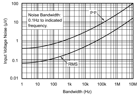
Figure 5-2. Total Input Voltage Noise vs Bandwidth
