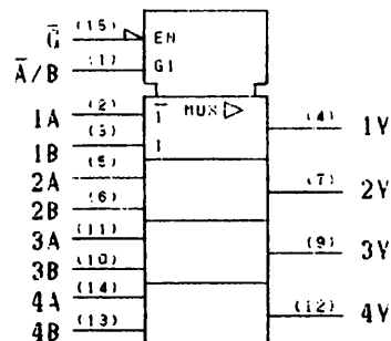
LOGIC SYMBOL
