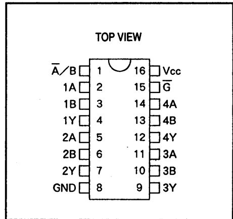
PIN ASSIGNMENT
