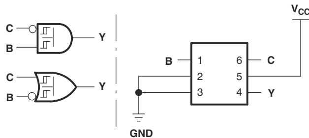
Figure 7-7. 14+08/14+02: 2-Input AND/NOR Gate With One Inverted Input
