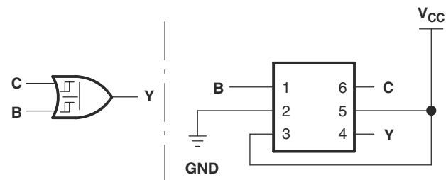
Figure 7-8. 32: 2-Input OR Gate
