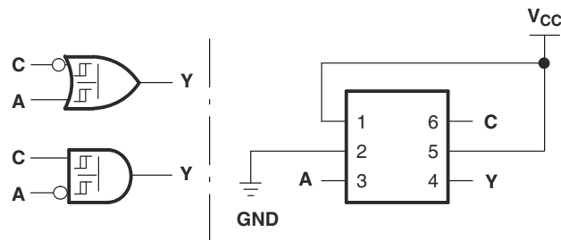
Figure 7-6. 14+32/14+00: 2-Input OR/NAND Gate With One Inverted Input
