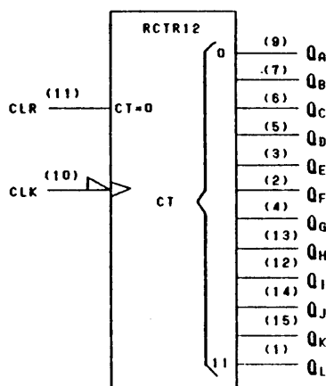
LOGIC SYMBOL
