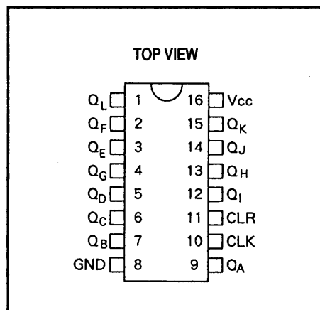
PIN ASSIGNMENT
