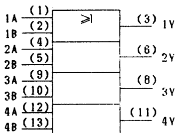
LOGIC SYMBOL
