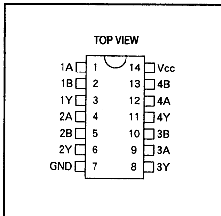
PIN ASSIGNMENT
