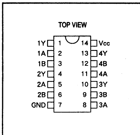
PIN ASSIGNMENT
