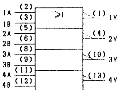
LOGIC SYMBOL.
