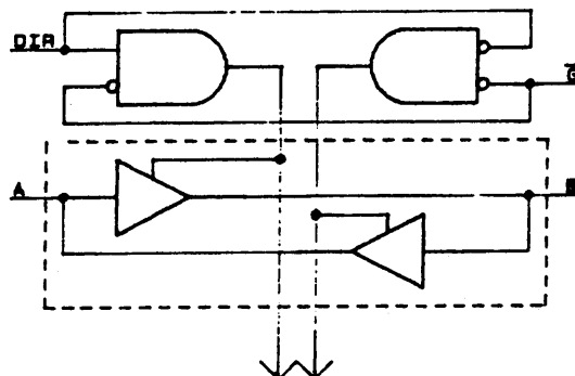
LOGIC DIAGRAM (1/8 CIRCUIT)
