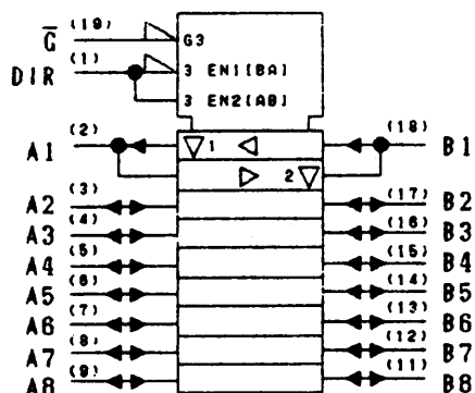
LOGIC SYMBOL
