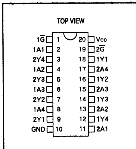
PIN ASSIGNMENT
