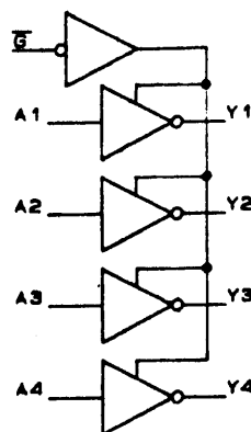
LOGIC DIAGRAM (1/2 CIRCUIT)
