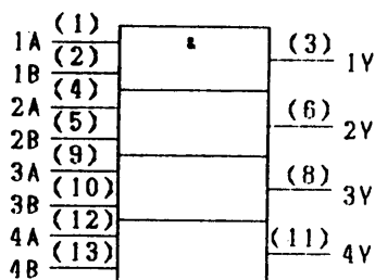
LOGIC SYMBOL
