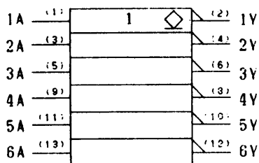
LOGIC SYMBOL
