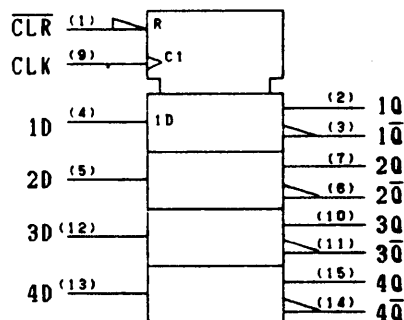
LOGIC SYMBOL
