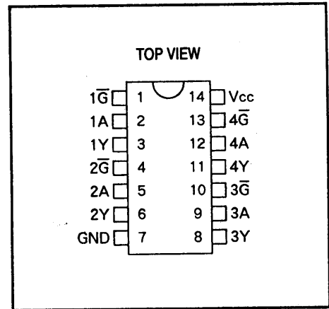
PIN ASSIGNMENT
