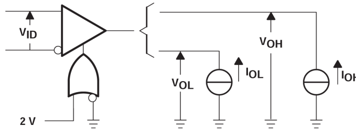
Figure 6-1. V_{OH} , V_{OL}
