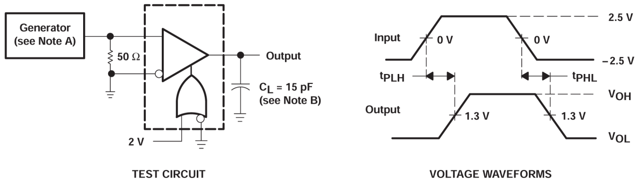
TEST CIRCUIT
