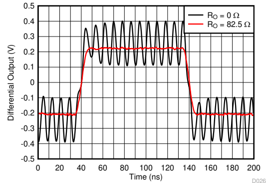
Figure 7-26. Step Response Into Capacitive Load
