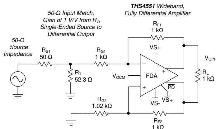
Figure 9-4. Single-Ended to Differential Gain of 1 V/V with Input Matching Using Standard Resistor Values
