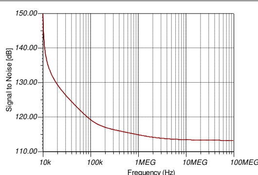
Figure 10-13. Signal-to-Noise Ratio Plot
