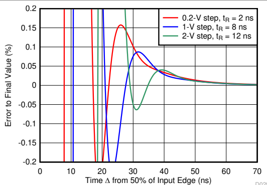
Figure 7-27. Small- and Large-Signal Step Response
