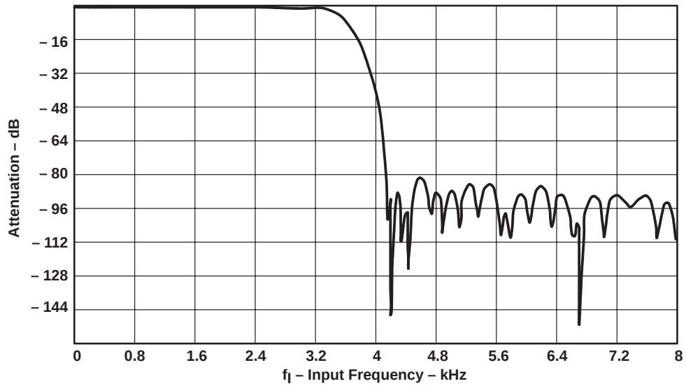
Figure 5-8. DAC Channel Filter Response (MCLK = 8.192 MHz, f_s = 8 kHz)
