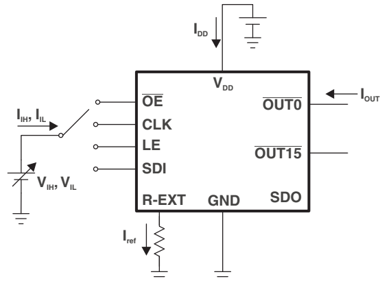
Figure 3. Test Circuit for Electrical Characteristics
