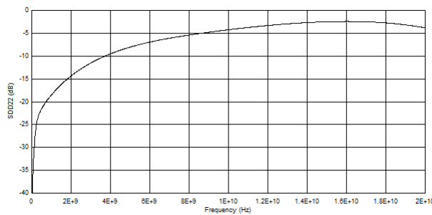
Figure 5-5. Output Differential Return Loss (SDD22)
