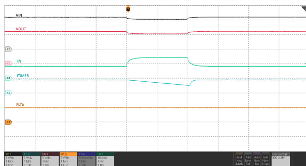
Figure 7-32. Inrush Current with Resistive and Capacitive Load
