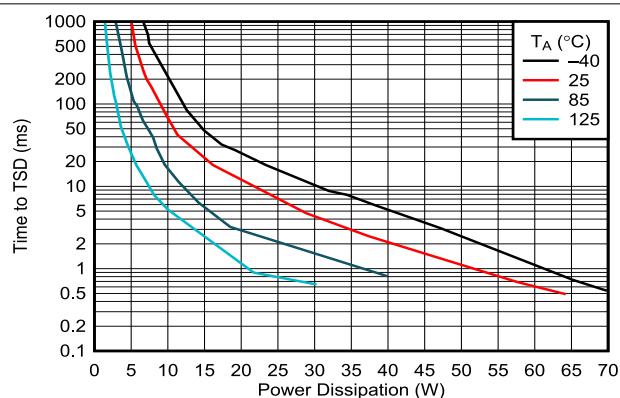
Figure 7-27. Time to Thermal Shutdown During Steady-State
