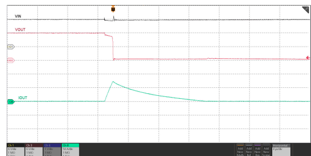
Figure 7-35. Circuit-Breaker Response
