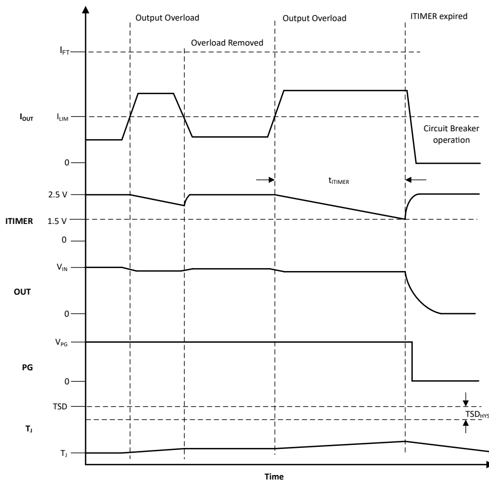
Figure 7-4. Circuit Breaker Response
