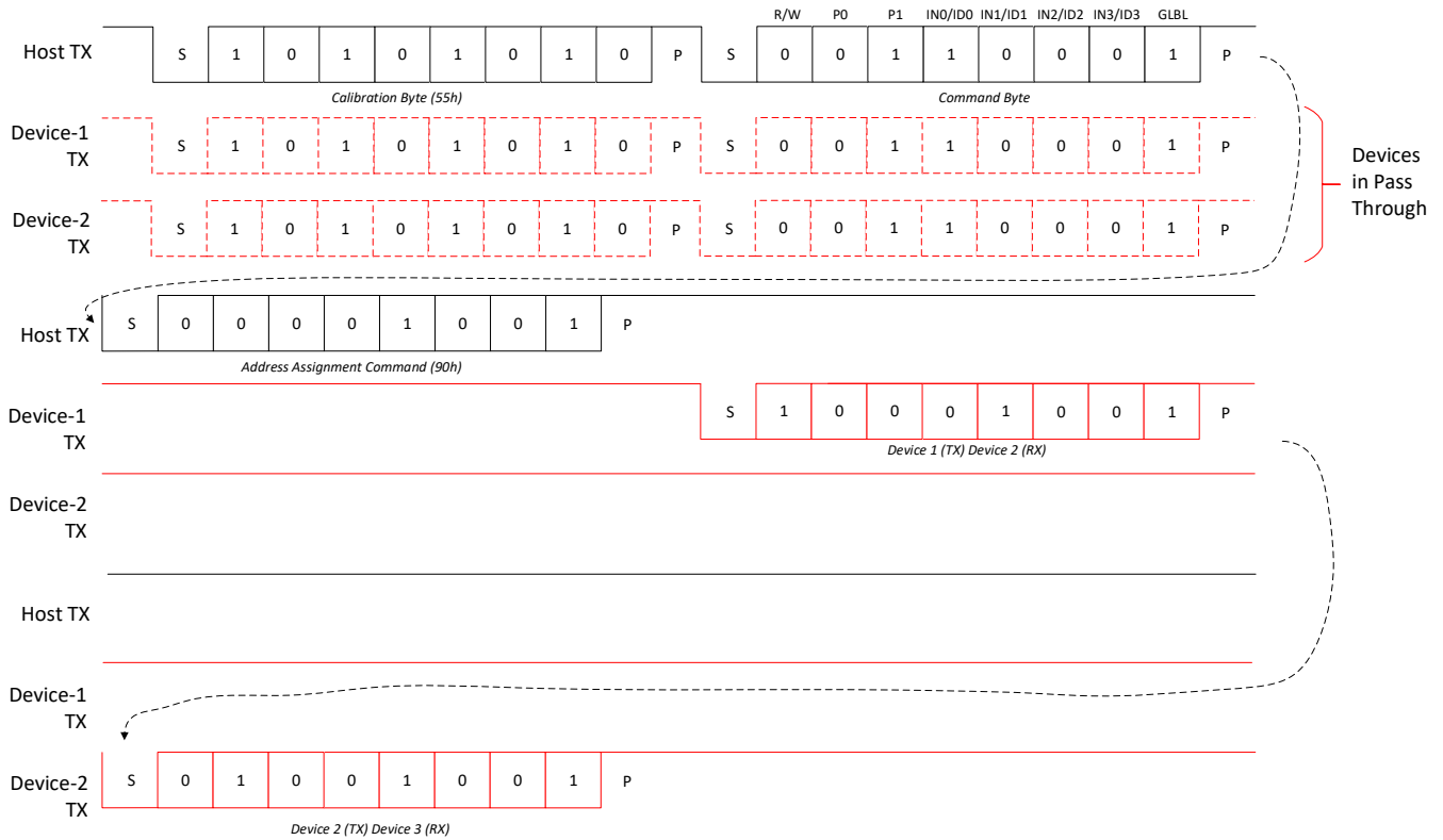
Figure 7-8. Global Initialization and Address Assignment Command Flow
