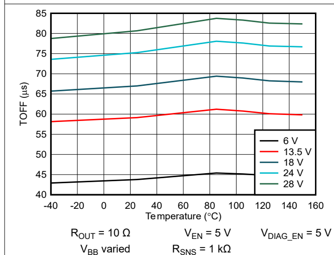
Figure 5-15. Turn off time T_{OFF} vs Temperature
