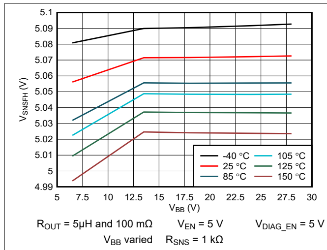
Figure 5-13. VSNSFH (5 V) vs VBB
