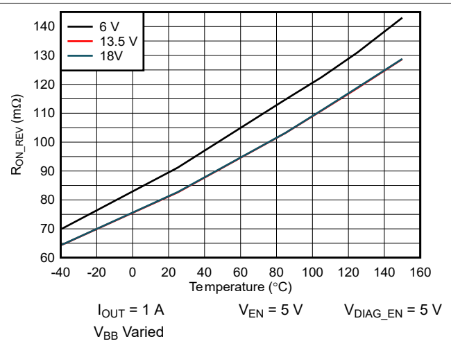
Figure 5-8. R_{ONREV} vs Temperature
