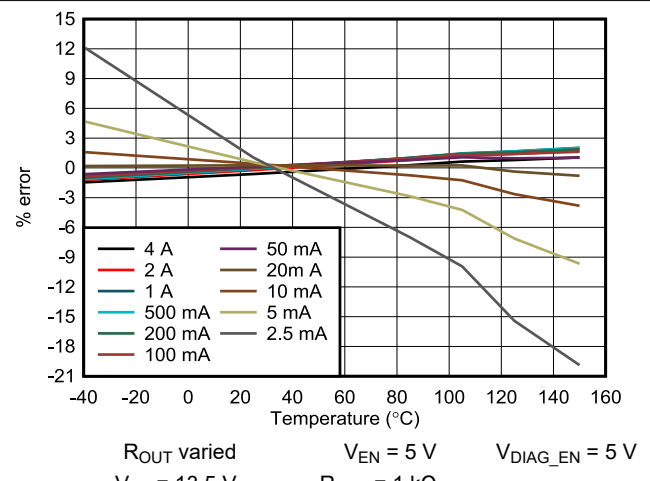
Figure 5-10. K_{SNS} Error vs Temperature
