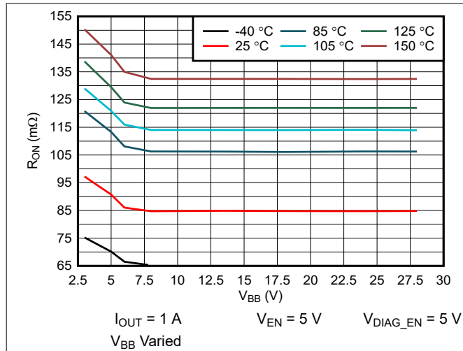
Figure 5-7. R_{DSON} vs V_{BB}
