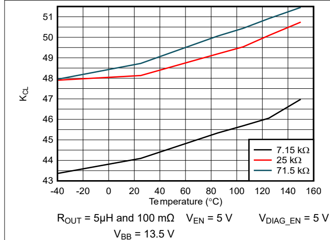
Figure 5-9. K_{CL} vs Temperature
