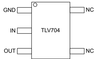
Figure 5-1. DBV Package, 5-Pin SOT-23 (Top View)
