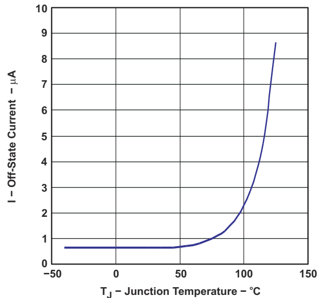
Figure 5-8. TPS2062-1, TPS2066-1 SUPPLY CURRENT, OUTPUT DISABLED vs JUNCTION TEMPERATURE
