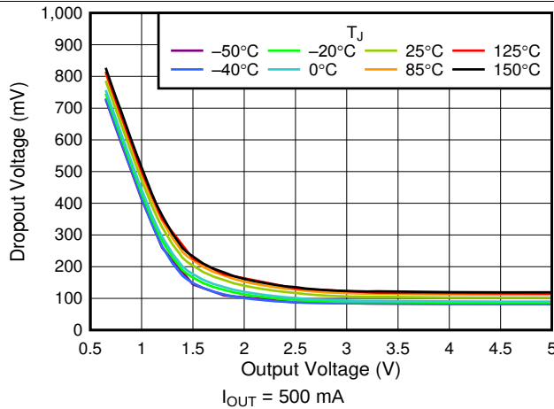
Figure 7. V_{DO} vs V_{OUT}
