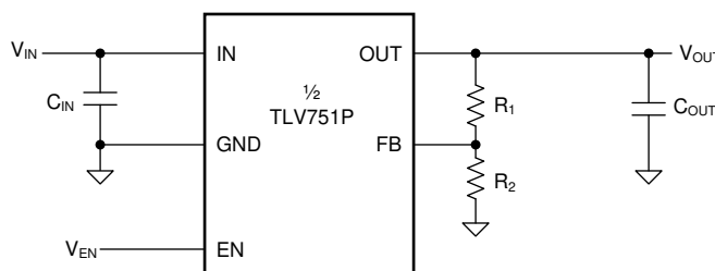
Figure 38. Adjustable Operation
