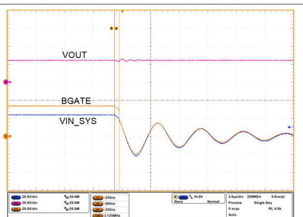
Figure 8-11. Input Hot-Short: Fast-Trip Response (Zoomed)
