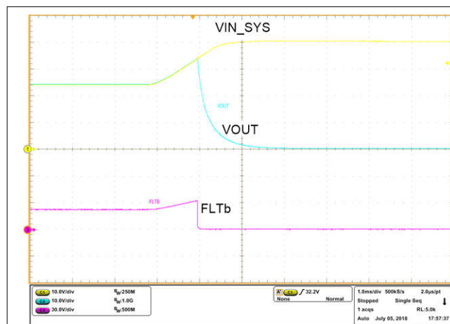
Figure 8-5. Overvoltage Cutoff Response at 33-V Level
