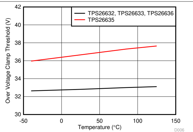
Figure 6-2. Overvoltage Clamp Threshold vs Temperature
