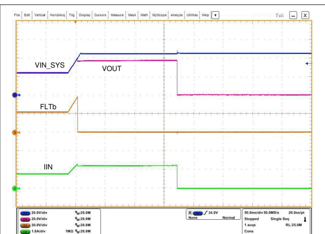
Figure 8-6. Overvoltage Clamp Response With TPS26635
