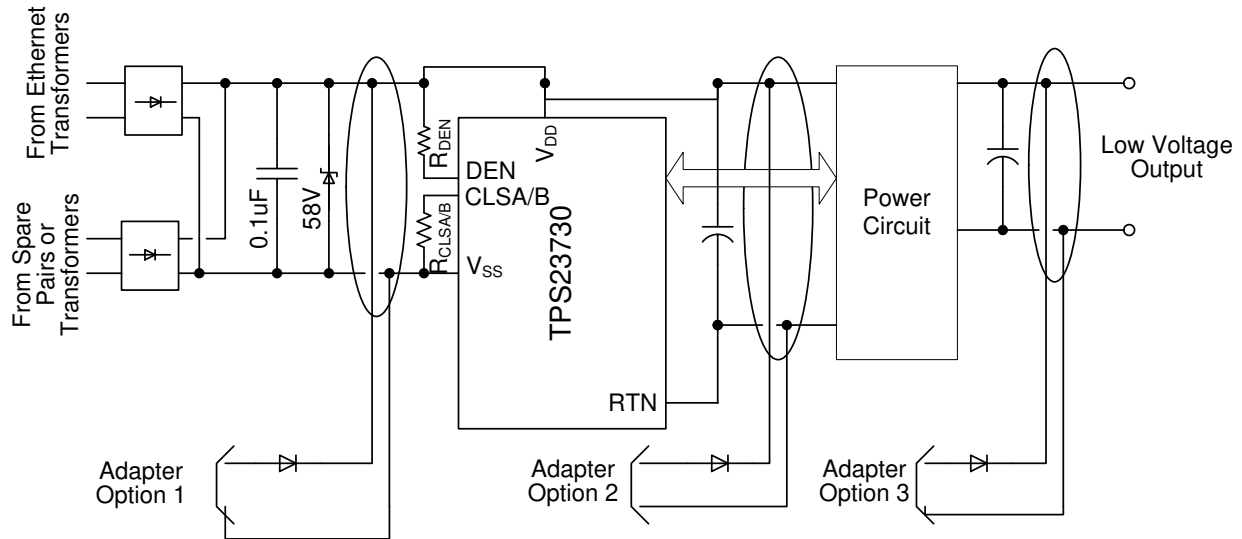
Figure 8-15. ORing Configurations
