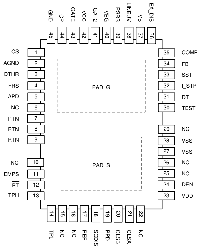
Figure 6-1. RMT Package 45-Pin VQFN Top View
