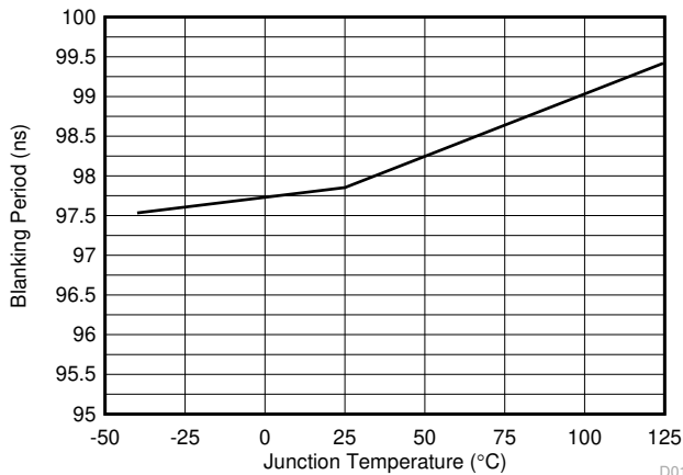
Figure 7-16. Blanking Period vs Temperature
