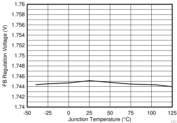
Figure 7-14. Feedback Regulation Voltage vs Temperature
